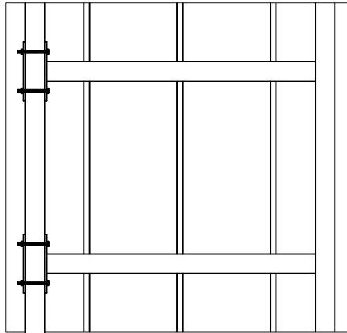
TYPE 2 CANTILEVER SIGN POST (RAILING) COMPLETE WITH M12 ST/ST BOLTS KITS
