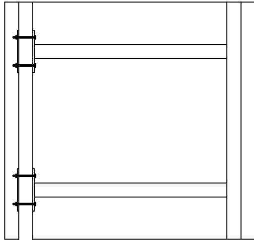
TYPE 2 CANTILEVER SIGN POST COMPLETE WITH M12 ST/ST BOLTS KITS
